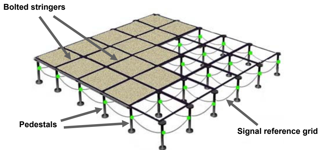
Figure 1 – Example of a signal reference grid
